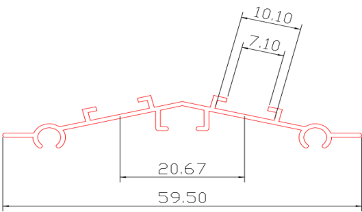
Aluminum LED profile (72 WATT)
