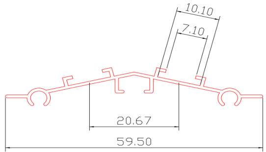
Polycarbonate Led profile (36 WATT)
